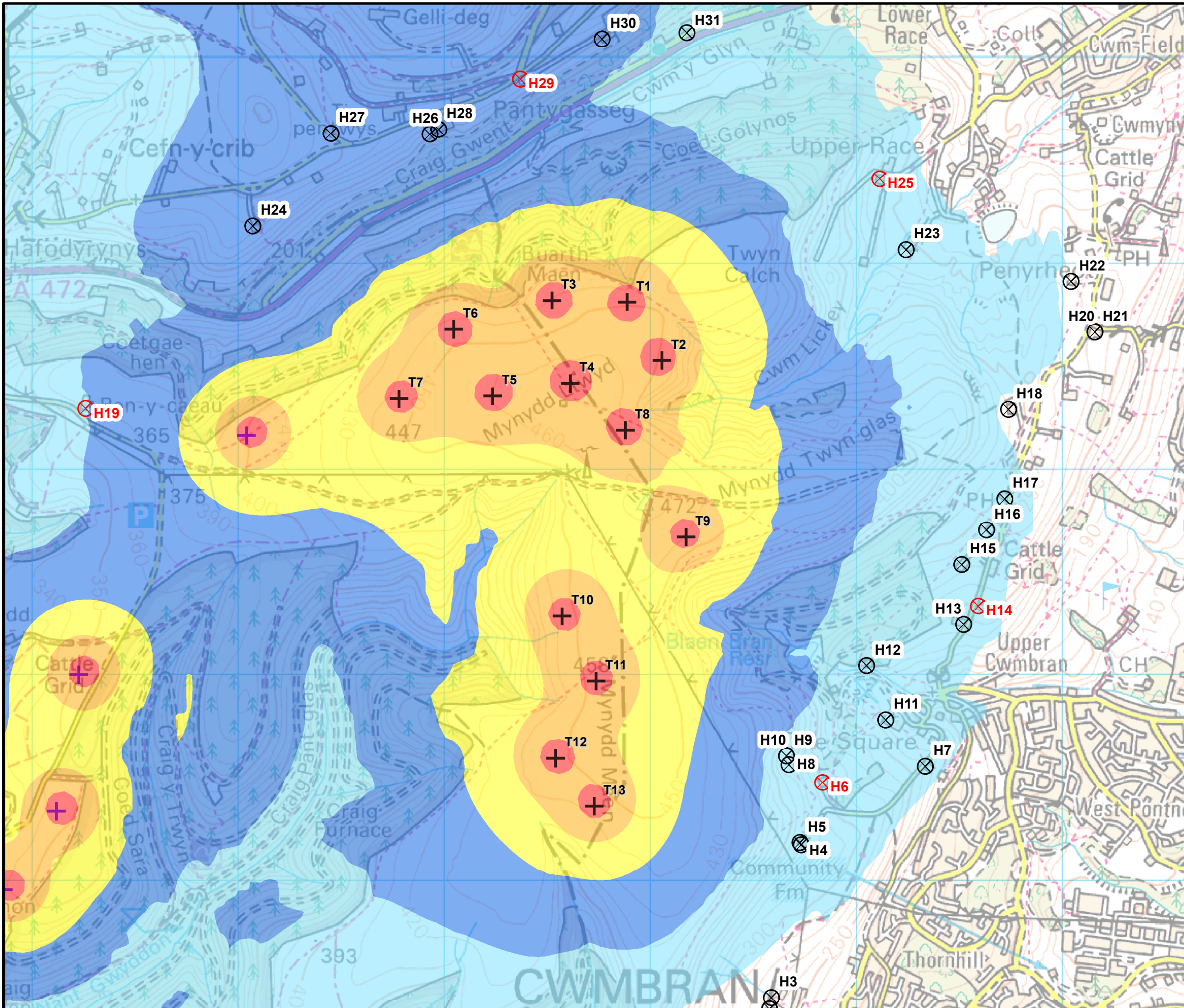
FIGURE 11.2 CUMULATIVE NOISE CONTOUR PLOT
