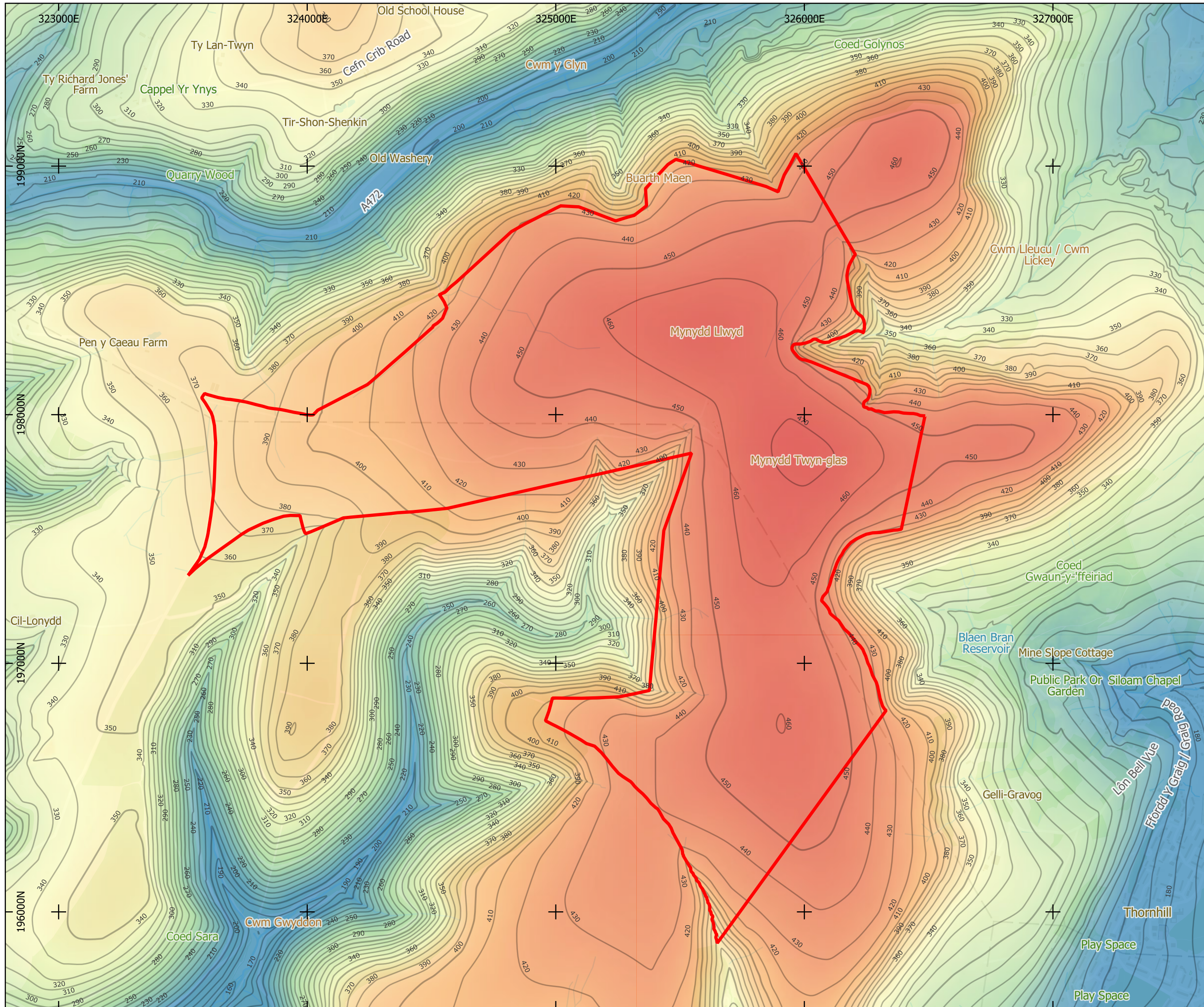
Mynydd Maen Wind Farm Figure 5 Topography of the Site Project No.07861A | 29/10/2023 | Drawn By: JM
