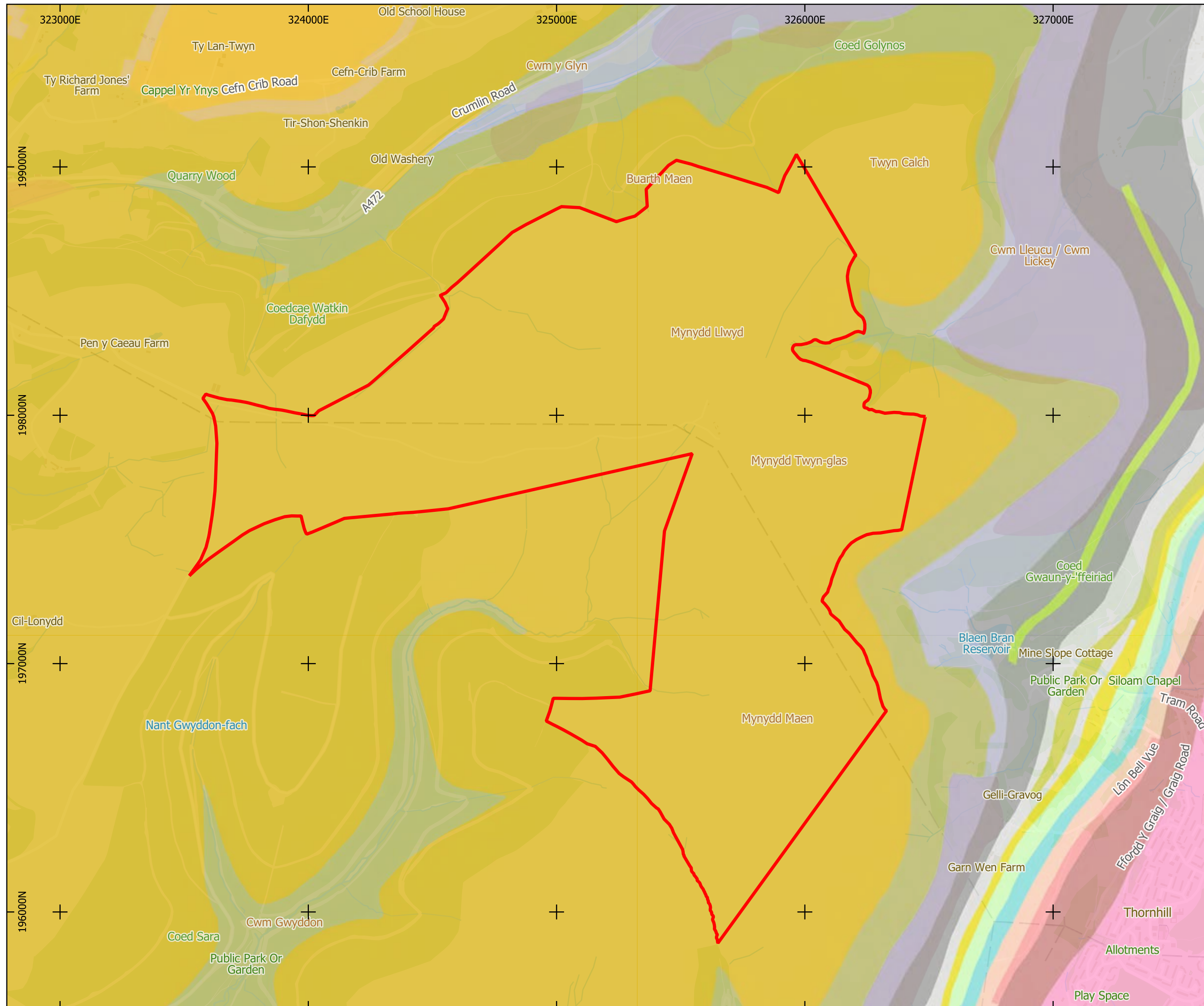
Mynydd Maen Wind Farm Figure 4 Geology of the Site Project No.07861A | 29/10/2023 | Drawn By: JM
